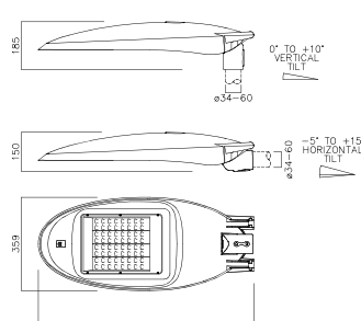
34-60MM FIXING (NO SUFFIX)
